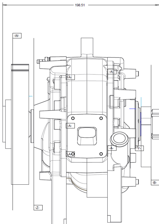
Rotapower 150 – Side View
