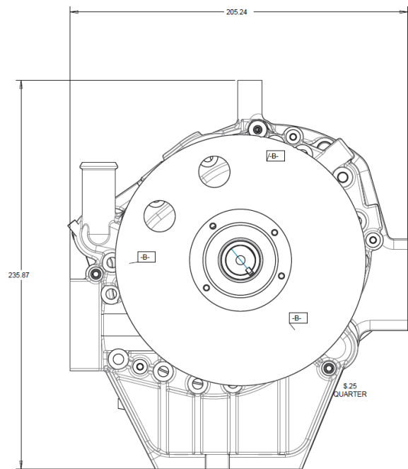
Rotapower 150 – End View
