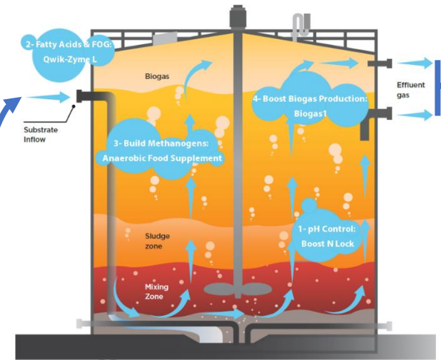
Anaerobic Digester
