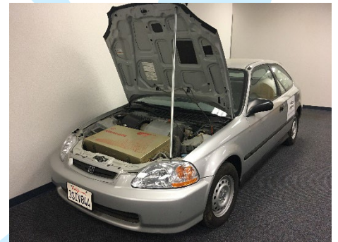
Hybrid car with 530cc Rotapower® engine in 0.94 Ft 3 lead lined enclosure producing 93 Kw
