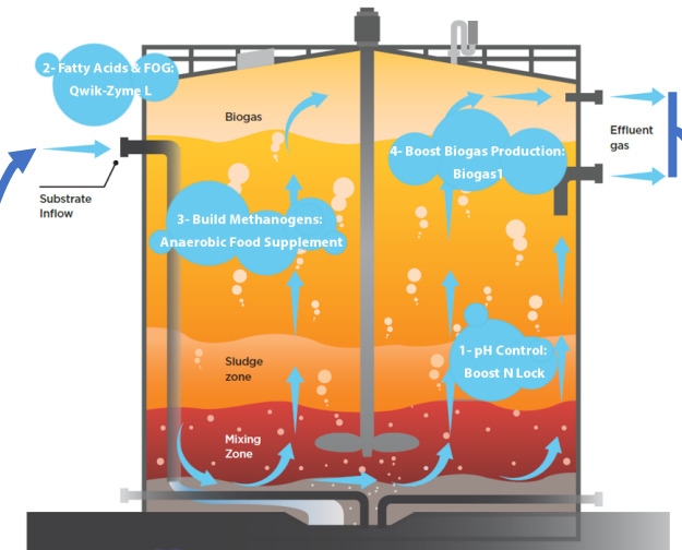
Anaerobic Digester
