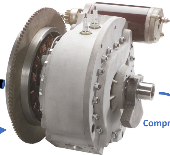
Rotapower® Compressor/Expander
